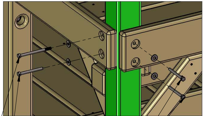
5/16" X 3-1/2" LAG SCREWS AND 5/16" WASHERS
