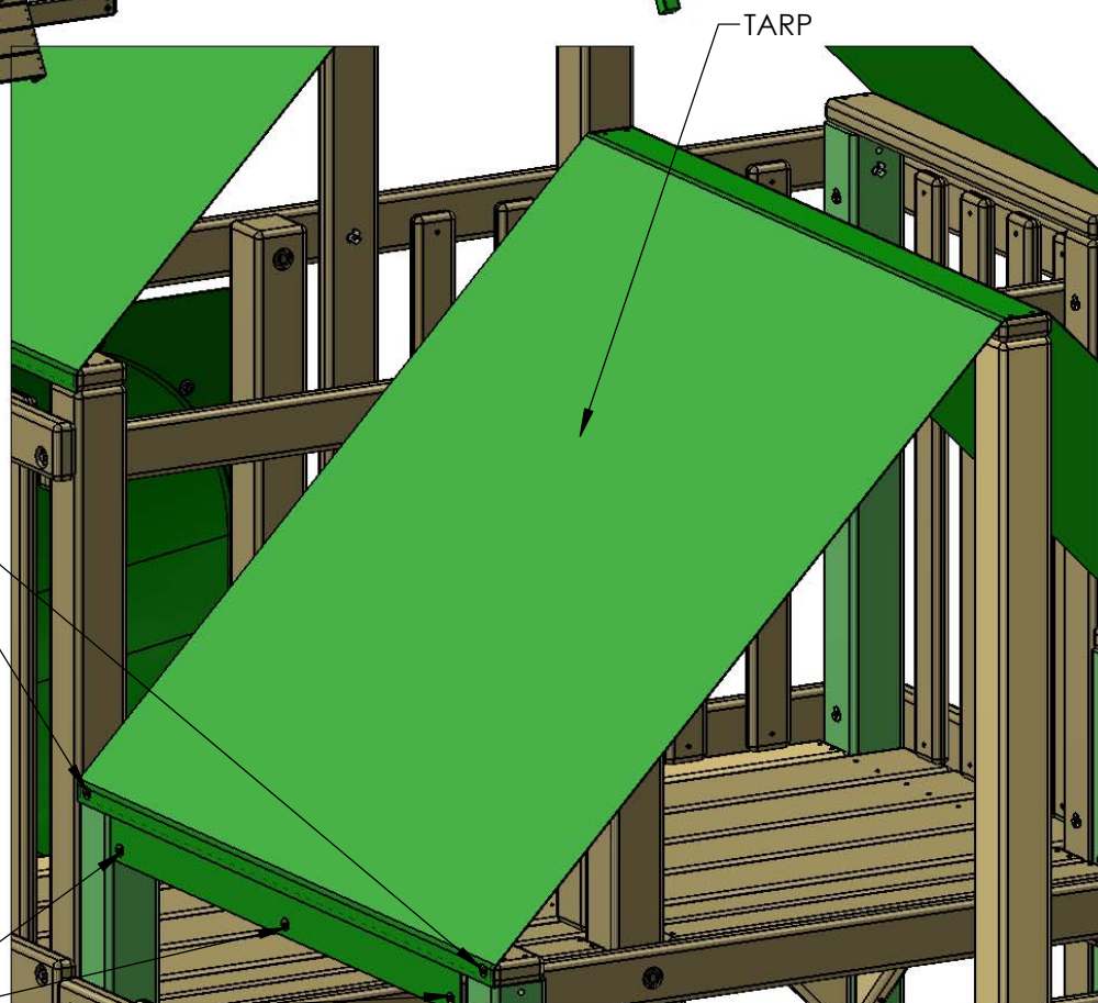
DETAIL A
