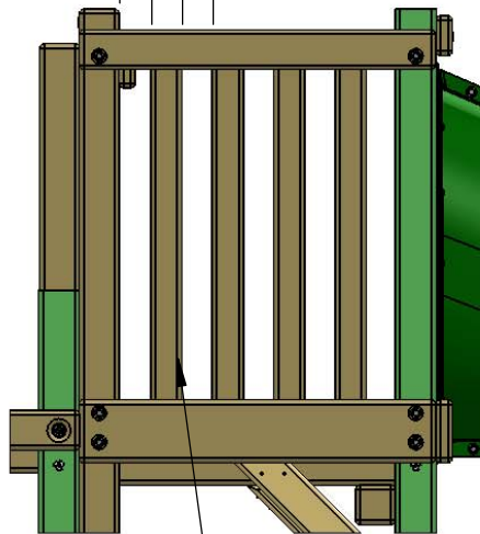
5/4 X 3 X 34-1/2" PANEL SLAT (4 ON RIGHT SIDE)
