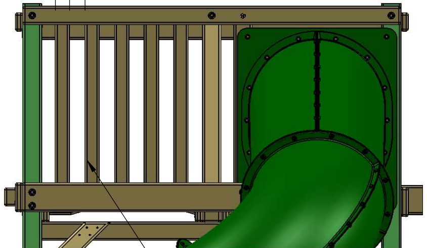
5/4 X 3 X 34-1/2" PANEL SLAT (5 ON REAR-RIGHT SIDE)
