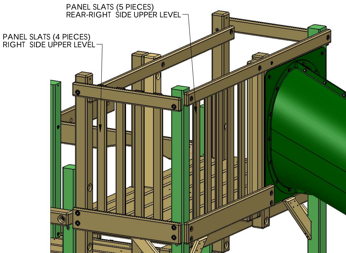
5/4 X 3 X 34-1/2" PANEL SLAT (4 ON RIGHT SIDE)
