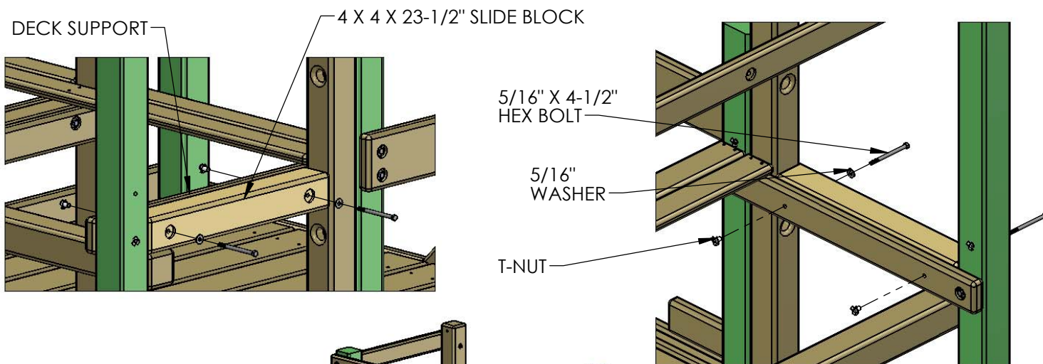
DETAIL A SCALE 2 : 25
