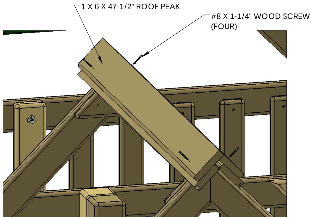
DETAIL A
